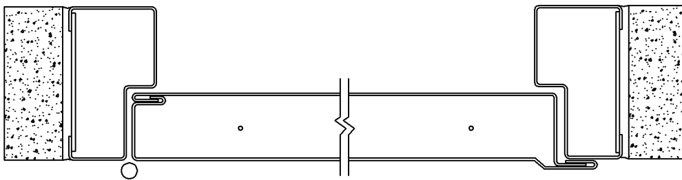
STANDARD ASTRAGAL
