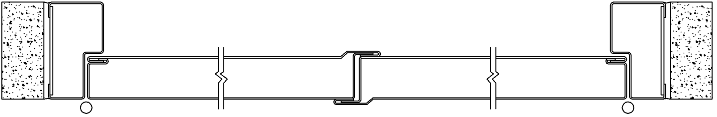
STANDARD ASTRAGAL
